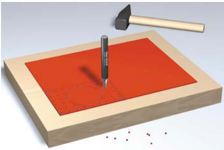
Abb. 6: Adaptermatte lochen
